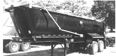
'16 MAC 28'x96"x60" trlr., center pt. susp., half round, 24.5 tires, steel whls., tdm., fixed axle, highlift tailgate, high tensile steel, stk. #2916-T, $42,900.
